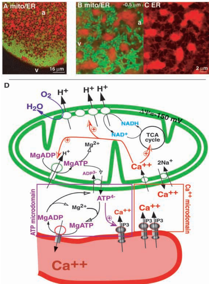
Fig. 5. Interactions between mitochondria and ER in the ascidian egg and in the \text{Ca}^{2+} and ATP microdomain. (A–C) Imaging of the ER network (red) and of mitochondria (green) in the vegetal contraction pole (v) of a fertilized Phallusia egg (A) shows the cortical ER-rich domain closely apposed to the subcortical mitochondria-rich domain. At higher resolution (B), rod-shaped mitochondria are observed densely packed in the vegetal subcortex ( 0.5\ \mu\text{m} under the surface of the egg). Mitochondria are in close proximity to ER-rich domains and tubes of ER (C; reveals ER tubes between ER-rich domains shown in B). a, animal side. (D) Probable \text{Ca}^{2+} fluxes in the \text{Ca}^{2+} microdomain forming at the interface between a mitochondria (green) and an ER tubule (red) with clustered \text{IP}_3\text{Rs} . In the same space an ATP microdomain is formed between mitochondria (producing and exporting ATP) and Mg-ATP-consuming pumps (SERCAs) and \text{ATP}^{4-} -using channels ( \text{IP}_3\text{Rs} ). Calcium released in the cytosol can be sequestered by the mitochondria where it stimulates oxidative phosphorylation. \text{ATP}^{4-} is exported from the mitochondria into the cytosol where it stimulates \text{Ca}^{2+} release by sensitizing the \text{IP}_3\text{Rs} to \text{Ca}^{2+} . Finally, Mg-ATP generated by mitochondria can energize \text{Ca}^{2+} pumping back into the ER lumen and replenish \text{Ca}^{2+} stores.
